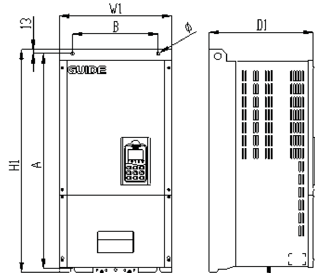
HF500A-4整流回馈模块外形尺寸:
